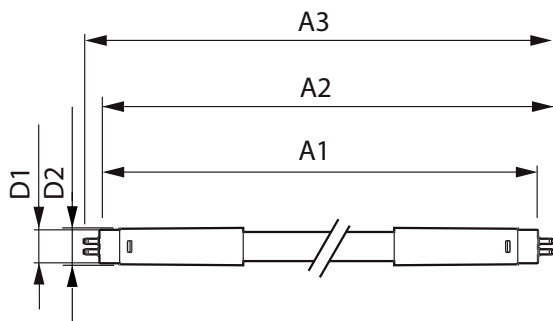
MAS LEDtube 1200mm HE 16.5W 840 T5
