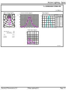
Accent Lighting Spots - CorePro LEDspot 4-50W GU10 827 36D DIM
