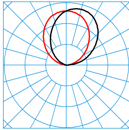
Sanesca W3 LED5000-840 01 (room light) TX055771 ■ C0 - C180 ■ C90 - C270 DIN 5040: E03 UTE: 0,00 J + 1,00 T CEN Flux Code: 0 0 0 0 100 50 81 96 100
