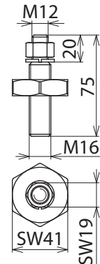
Maßbild AS SCHR M16 55 M12
