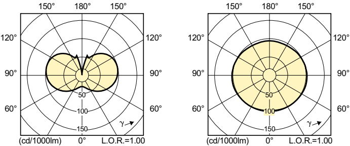
Light Distribution Diagram - MASTER CityWh CDO-TT Plus 50W/828 E27
