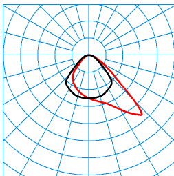
Bicult Act T SMS TGCS 5500 QI 05 EU (ActDCW) TX122142 ■ C0 - C180 ■ C90 - C270 DIN 5040: A50 UTE: 1,00 D CEN Flux Code: 59 89 98 100 100 0 0 0 0
