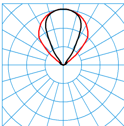
Bicult Act T SMS TGCS 5500 QI 05 EU (ActICW) TX122124 ■ C0 - C180 ■ C90 - C270 DIN 5040: E04 UTE: 0,00 J + 1,00 T CEN Flux Code: 0 0 0 0 100 82 96 100 100
