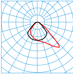
Bicult Act T SMS TGCS 5500 QI 05 EU (ActDWW) TX122138 ■ C0 - C180 ■ C90 - C270 DIN 5040: A50 UTE: 1,00 D CEN Flux Code: 59 89 98 100 100 0 0 0 0
