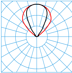
Bicult Act T SMS TGCS 5500 QI 05 EU (ActIWW) TX122137 ■ C0 - C180 ■ C90 - C270 DIN 5040: E04 UTE: 0,00 J + 1,00 T CEN Flux Code: 0 0 0 0 100 82 96 100 100
