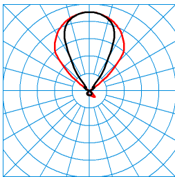
Bicult Act T SMS TGCS 5500 QI 05 EU (ActCCW) TX122121 ■ C0 - C180 ■ C90 - C270 DIN 5040: D54 UTE: 0,10 D + 0,90 T CEN Flux Code: 59 89 98 10 100 82 96 100 90
