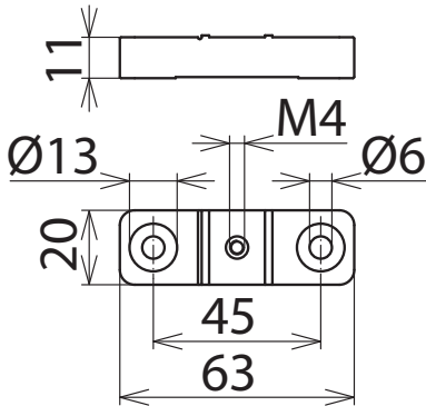
Maßbild ST AS SAK K
