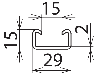
Maßbild AS SAK 1000 V2A
